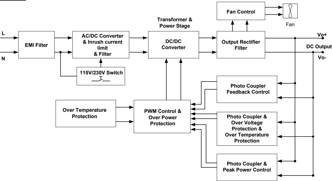
PMT-□V350W2BR□
