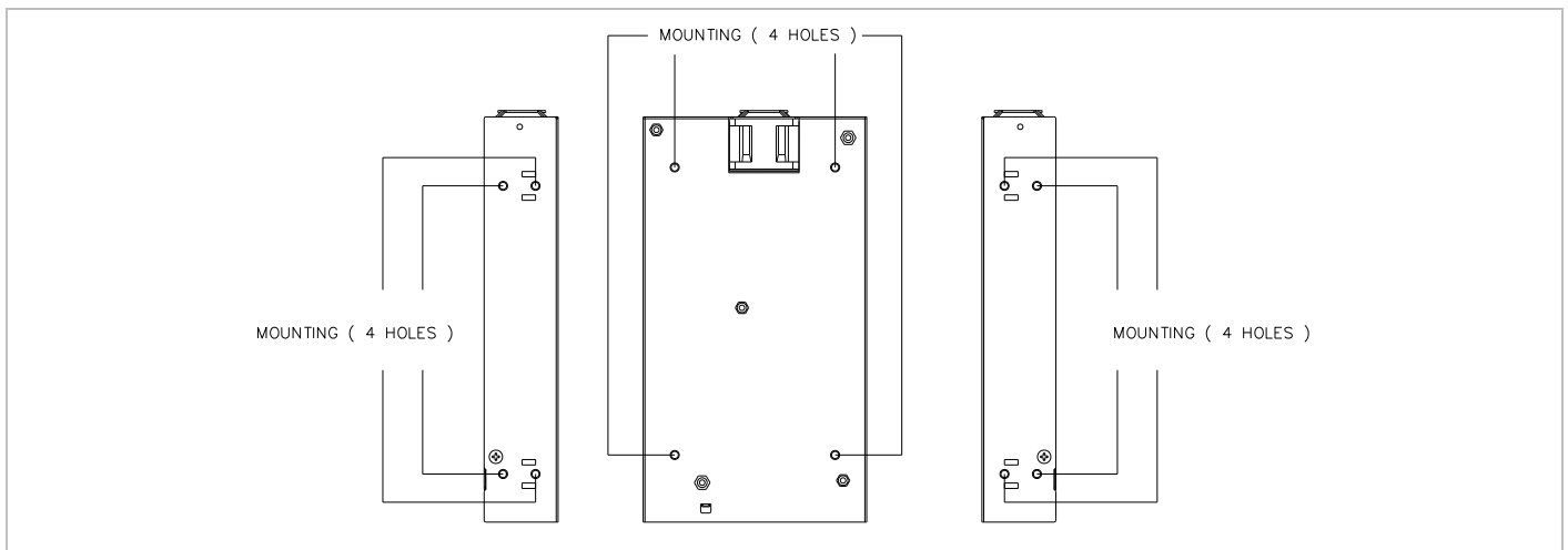
Fig. 3 Assembly Reference
