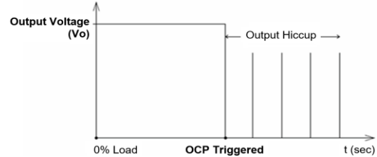
Figure 3. Hiccup at OLP/OCP
