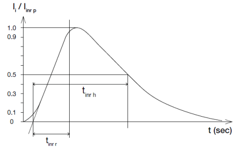
Figure 6. Inrush Current
