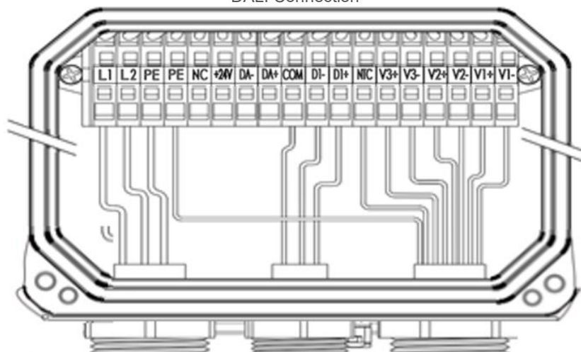
RDM/DMX Connection
