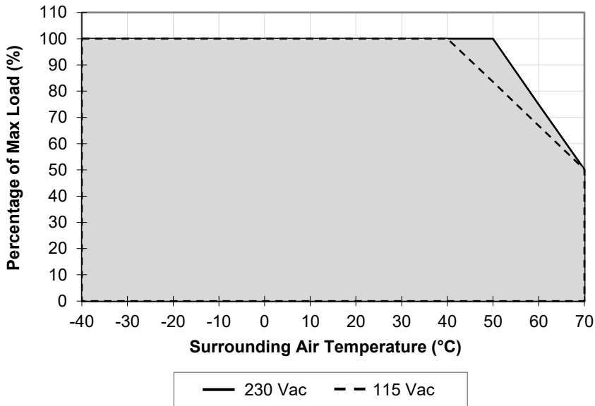
Fig. 1 De-rating for Vertical Mounting Orientation > 50°C de-rate power by 2.5 % / °C @ 230 Vac > 40°C de-rate power by 1.66 % / °C @ 115 Vac
