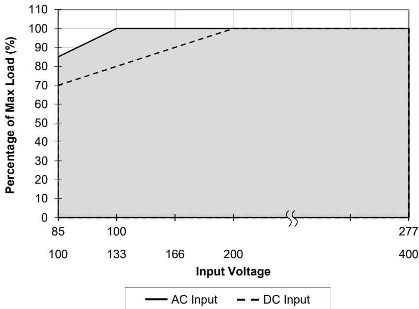
Fig. 2 De-rating for AC & DC Input Voltage < 100 Vac de-rate power by 1% / Vac < 200 Vdc de-rate power by 0.3% / Vdc
