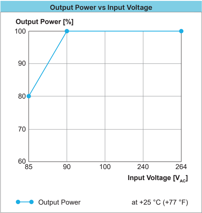
Fig. 19: Output power versus input voltage for W1AC-xxDC-150W-IN-nF
