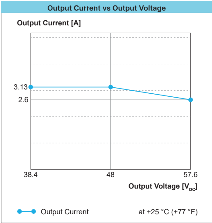
Fig. 22: Output current versus output voltage for W1AC-48DC-150W-IN-nF
