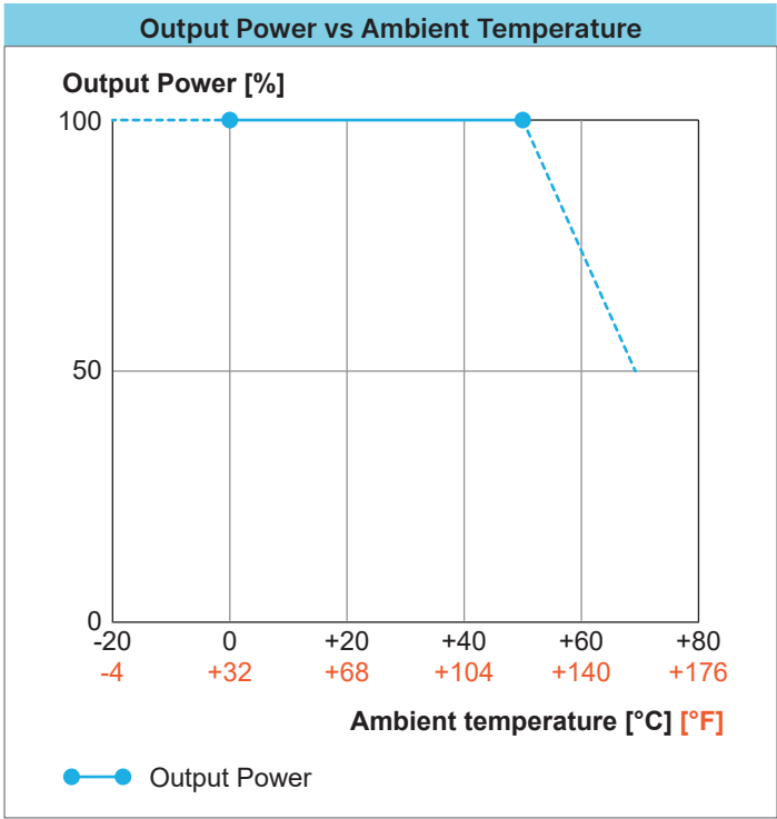
Fig. 20: Output power versus ambient temperature for W1AC-xxDC-150W-IN-nF
