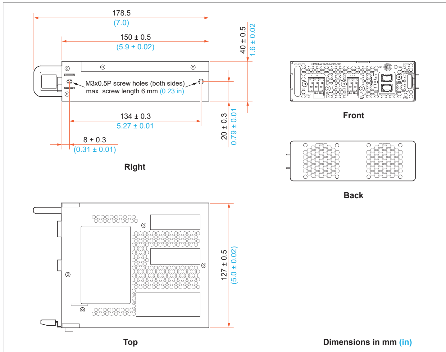
Fig. 17: Dimensions
