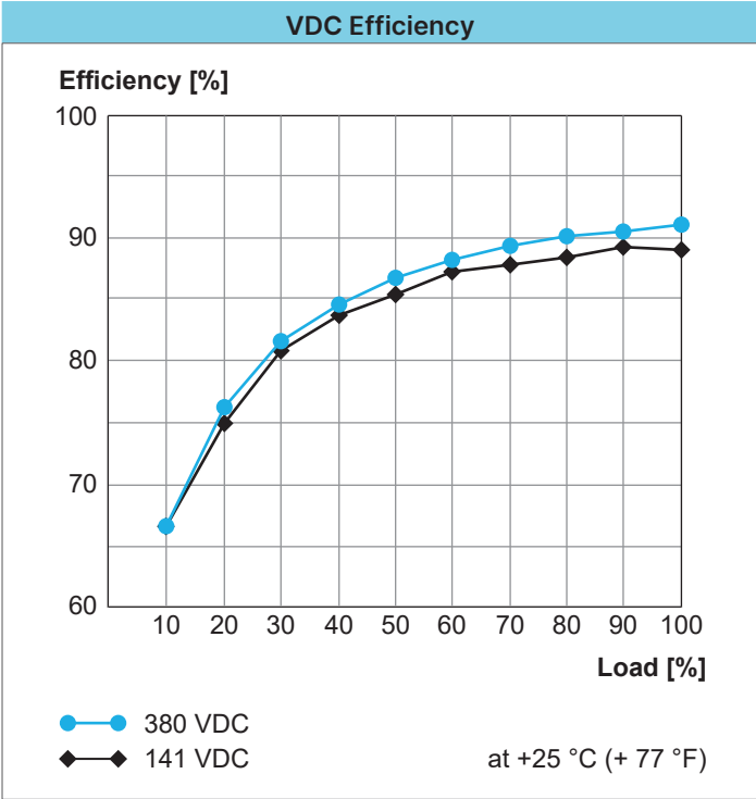
Fig. 24: VDC Efficiency for W1AC-24DC-150W-IN-nF
