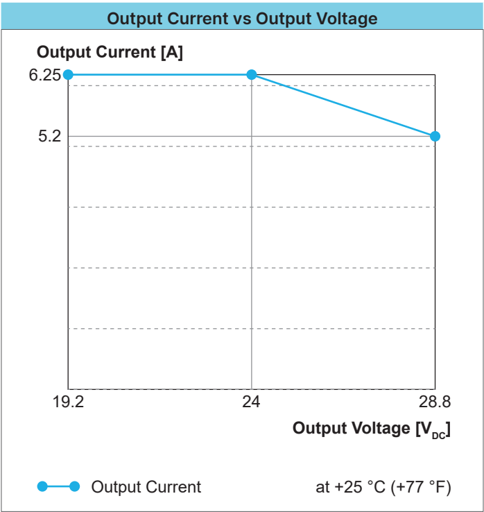
Fig. 21: Output current versus output voltage for W1AC-24DC-150W-IN-nF
