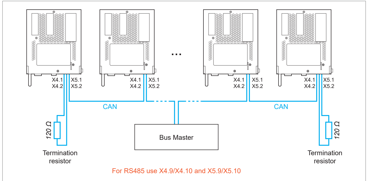
Fig. 25: Use of termination resistors in CAN / RS485 bus
