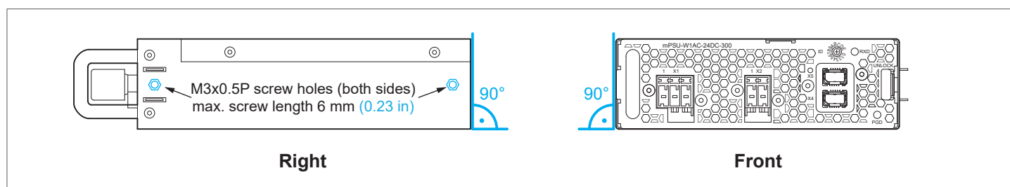
Fig. 18: Mounting orientations
