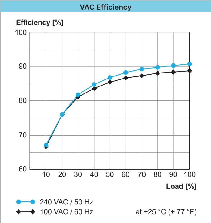
Fig. 23: VAC Efficiency for W1AC-24DC-150W-IN-nF
