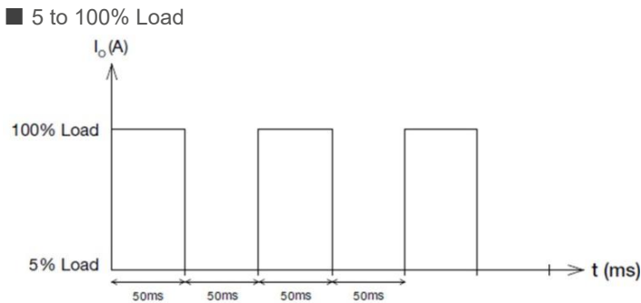
Figure 6. Dynamic Load
