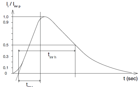
Figure 7. Inrush Current
