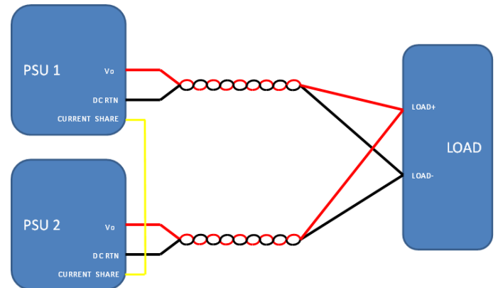
Fig. 10: Parallel connection
