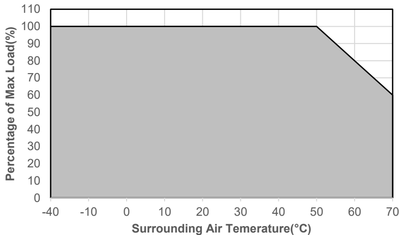
Fig. 1 De-rating for Horizontal Mounting Orientation > 50°C de-rate power by 2.0% / °C
