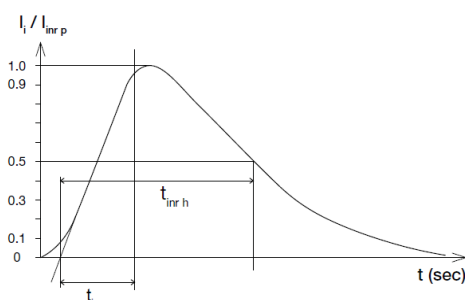
Fig. 7 Inrush Current
