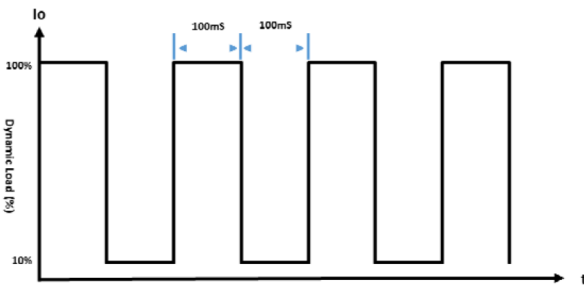
Figure 3-1. Dynamic Load (5 Hz)
