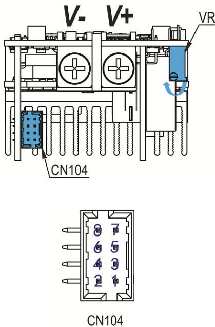
Fig. 17: -x2 Module connector
