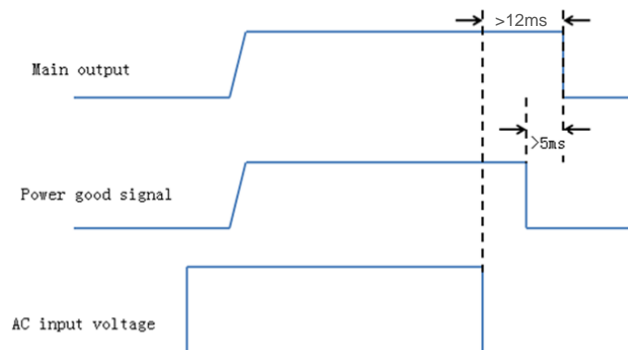
Fig. 27: Power good signal sequence
