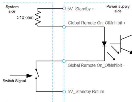
Fig. 32: Global Remote On_off connection
