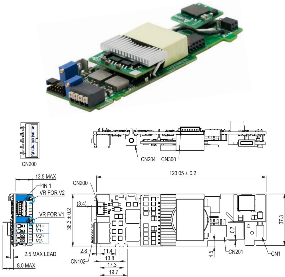
Fig. 9: Dimensional drawing Single Slot Dual Output Module
