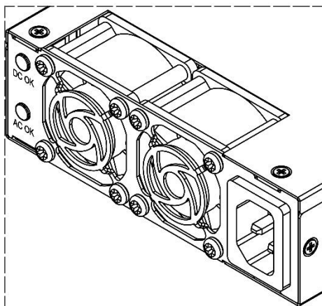
Figure 10. IEC320-C14
