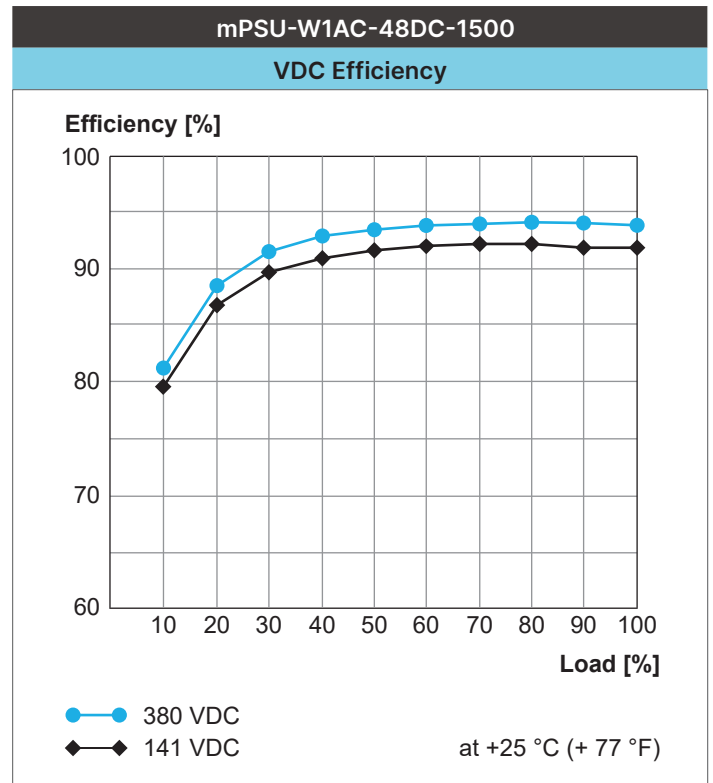
Fig. 12: VDC Efficiency for W1AC-48DC
