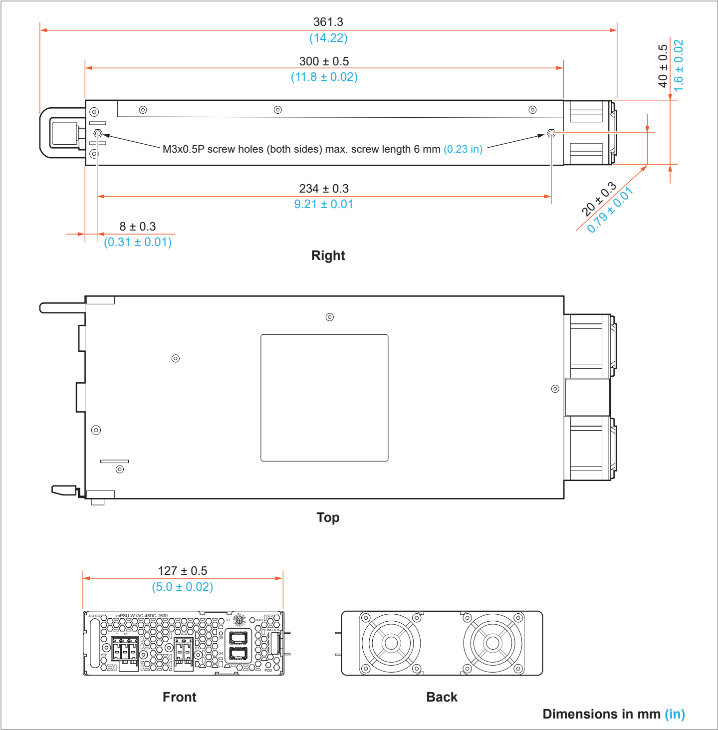
Fig. 6: Dimensions
