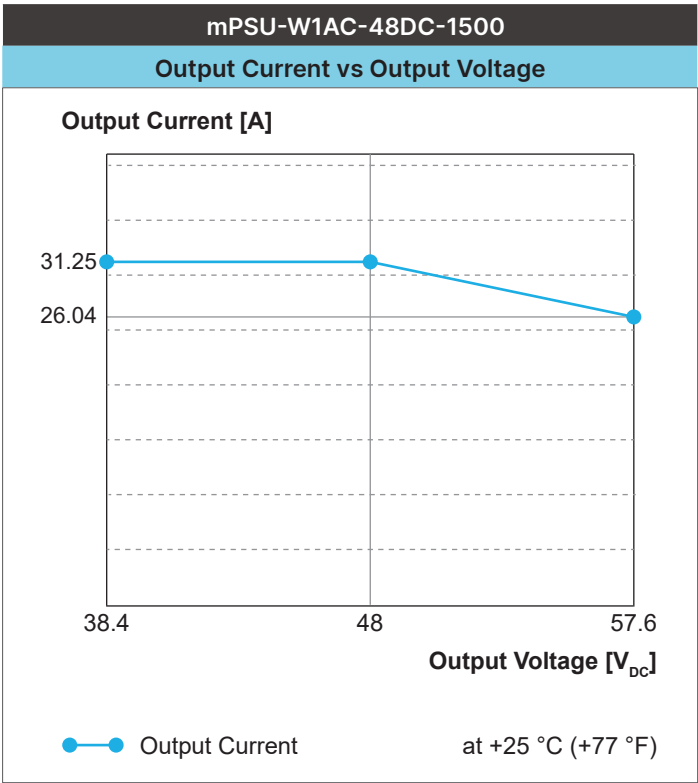
Fig. 10: Output current versus output voltage for W1AC-48DC
