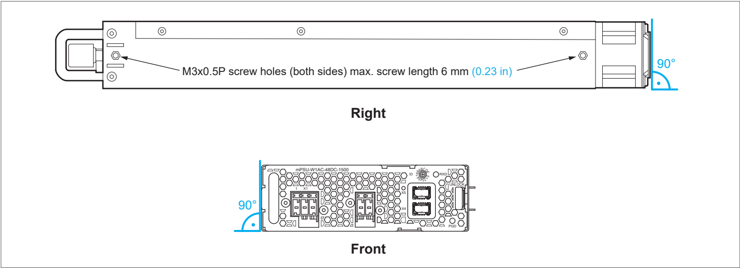
Fig. 7: Mounting orientations
