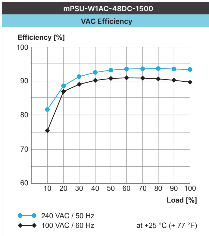
Fig. 11: VAC Efficiency for W1AC-48DC
