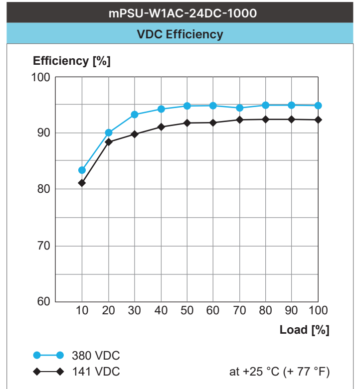
Fig. 13: VDC Efficiency for W1AC-24DC
