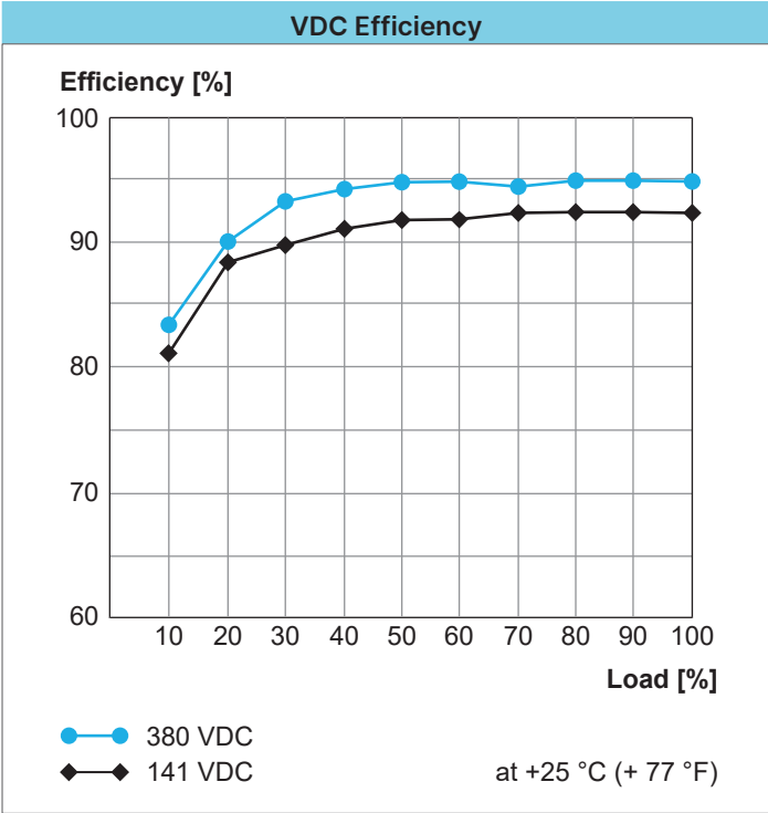
Fig. 24: VDC Efficiency for W1AC-24DC-1000W
