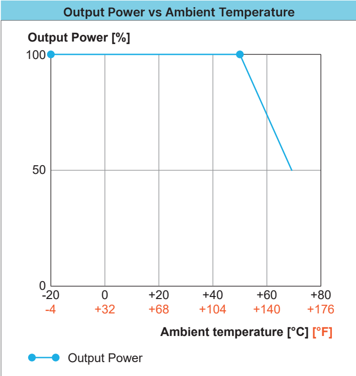
Fig. 20: Output power versus ambient temperature for W1AC-xxDC-1000W
