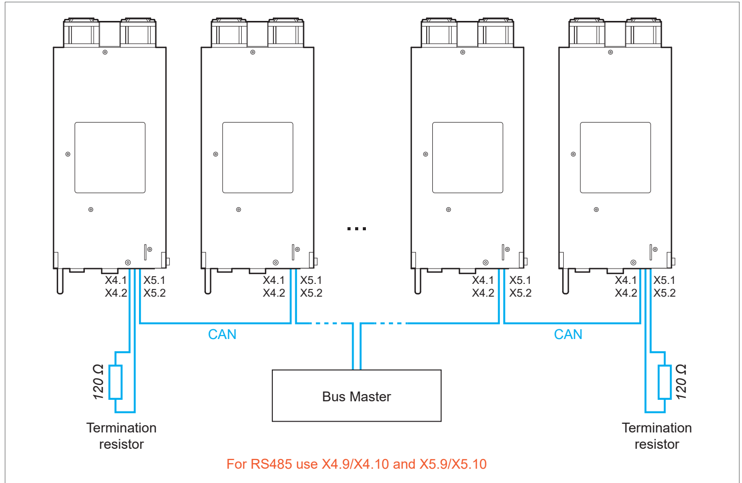
Fig. 27: Use of termination resistors in CAN / RS485 bus
