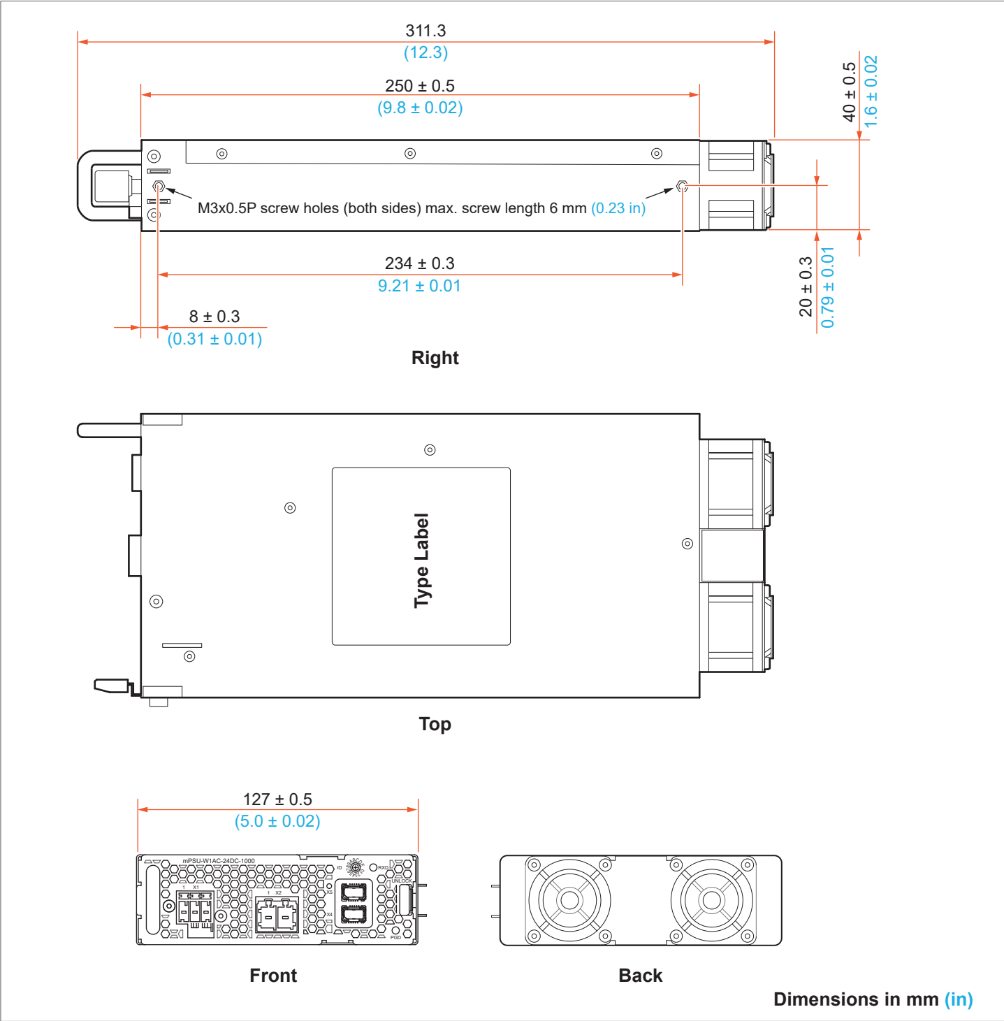
Fig. 17: Dimensions
