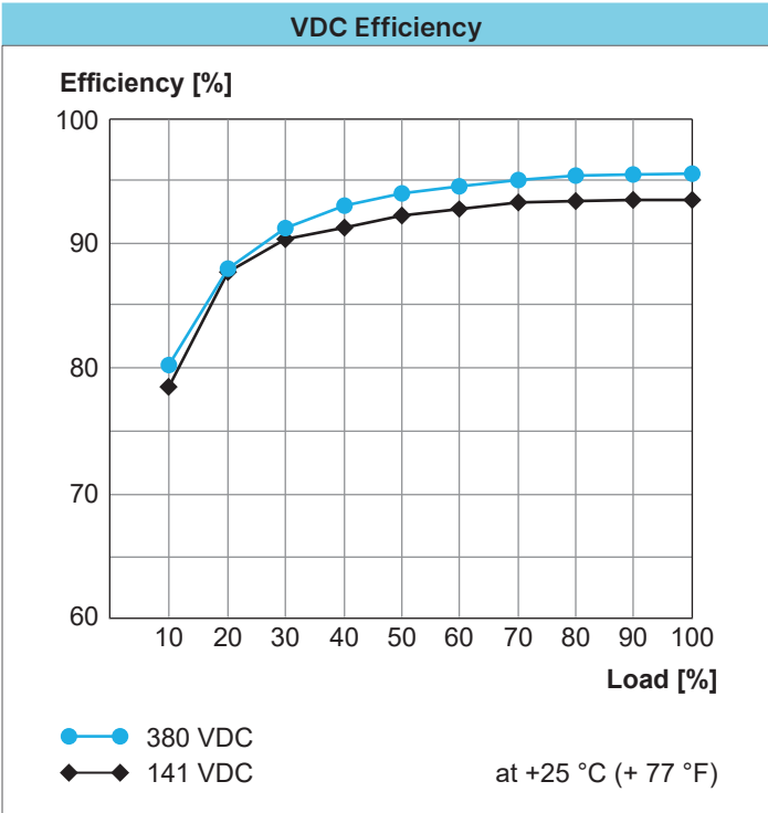
Fig. 26: VDC Efficiency for W1AC-48DC-1000W
