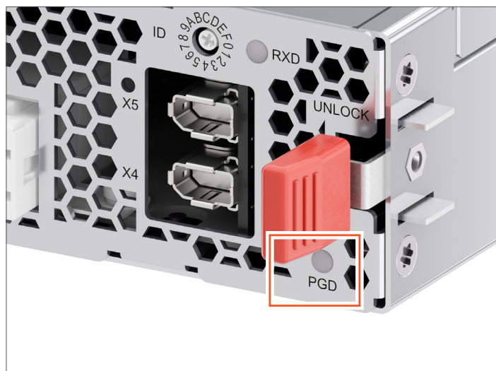
Fig. 7: PGD LED
