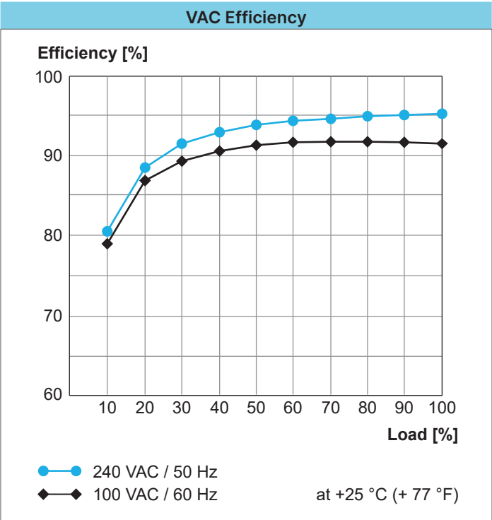
Fig. 25: VAC Efficiency for W1AC-48DC-1000W
