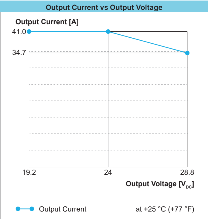
Fig. 21: Output current versus output voltage for W1AC-24DC-1000W
