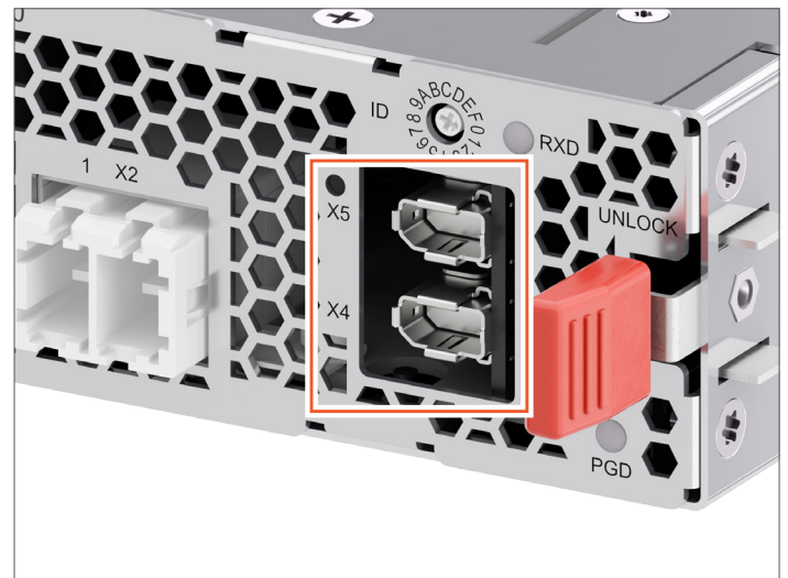
Fig. 4: Power Management Interface (X4, X5)
