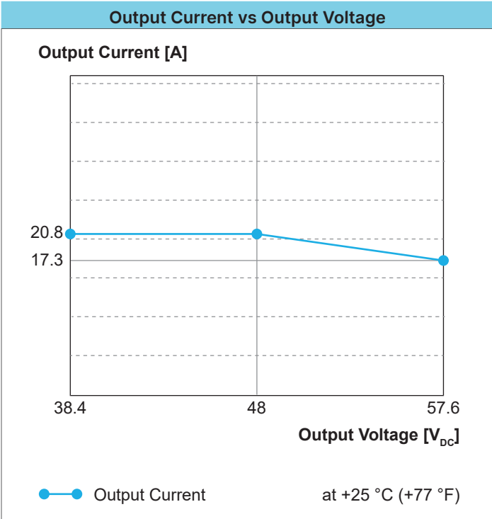
Fig. 22: Output current versus output voltage for W1AC-48DC-1000W
