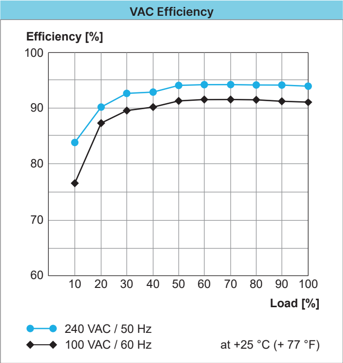
Fig. 23: VAC Efficiency for W1AC-24DC-1000W
