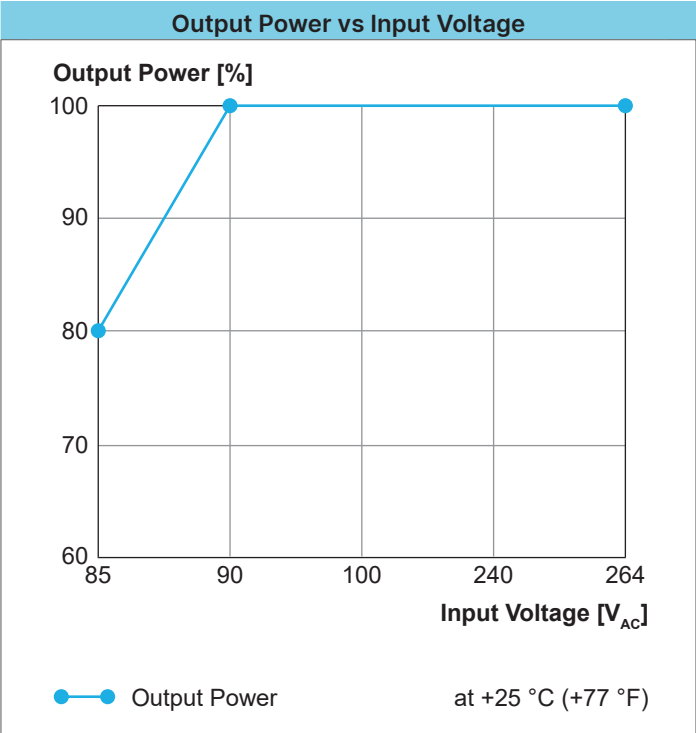
Fig. 19: Output power versus input voltage for W1AC-xxDC-1000W
