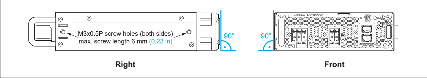
Fig. 18: Mounting orientations
