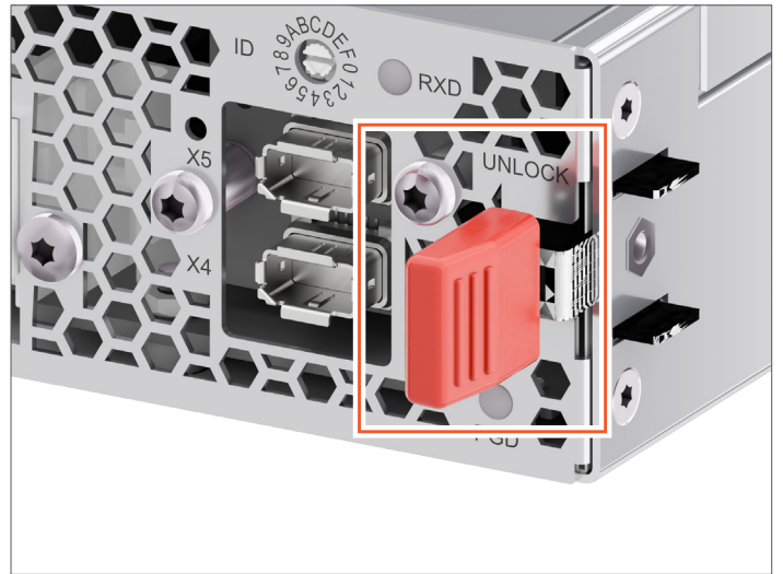
Fig. 8: Unlock Lever
