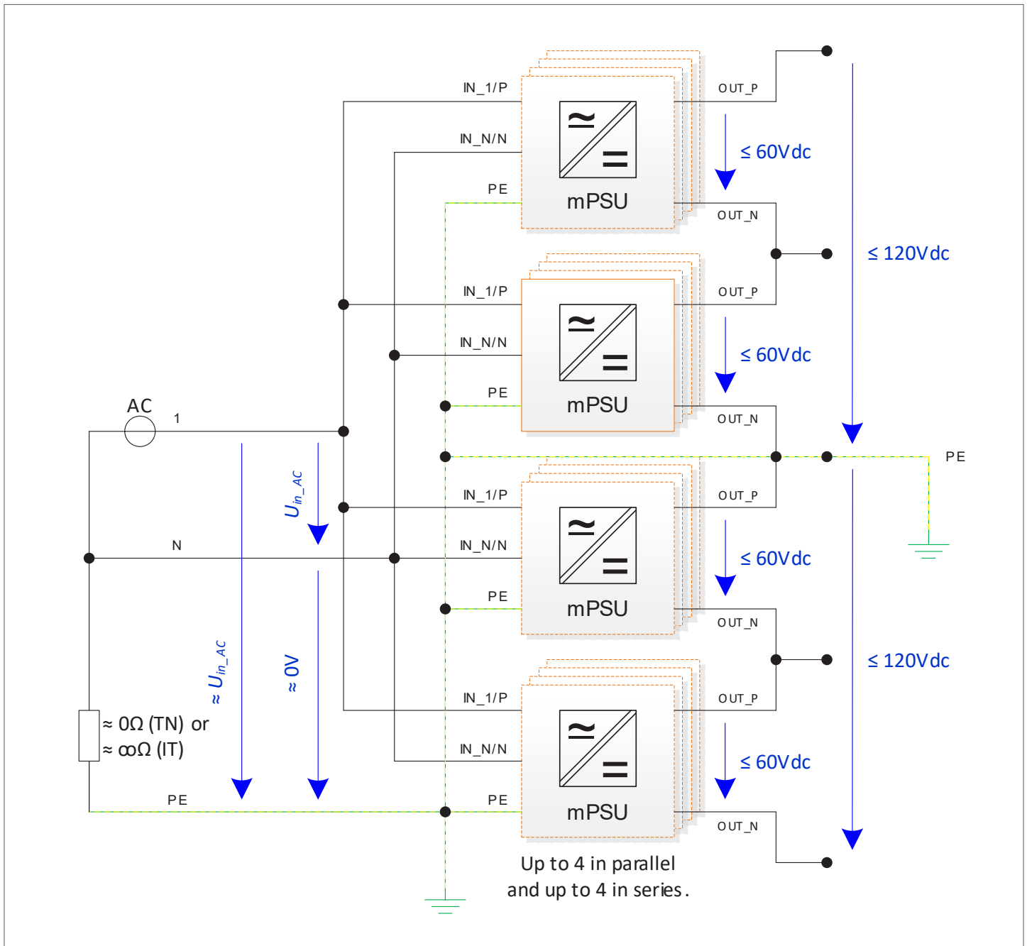
Fig. 11: System interoperability W1AC, 1-phase AC mains
