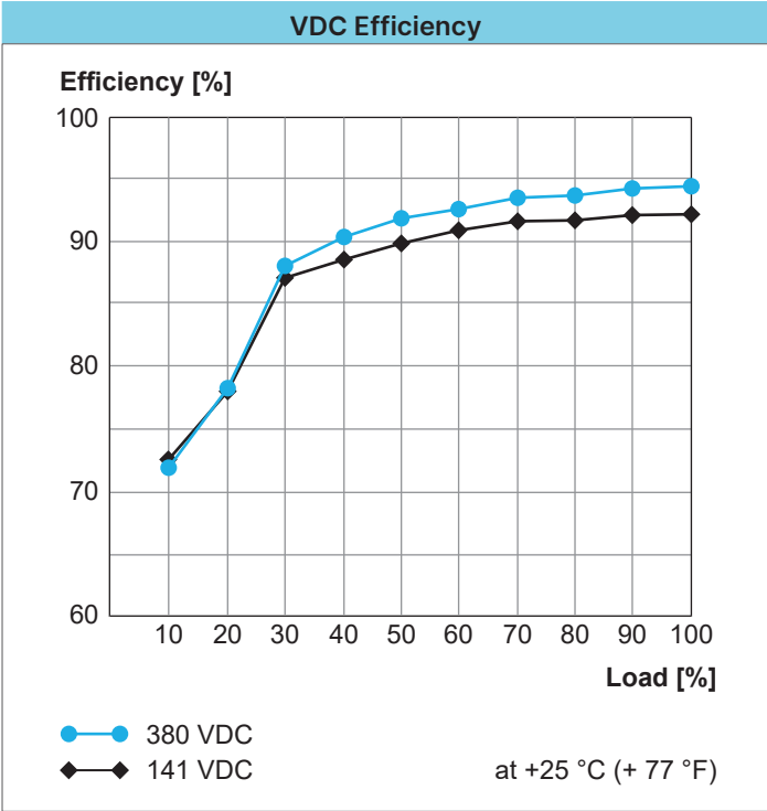
Fig. 24: VDC Efficiency for W1AC-24DC-300W
