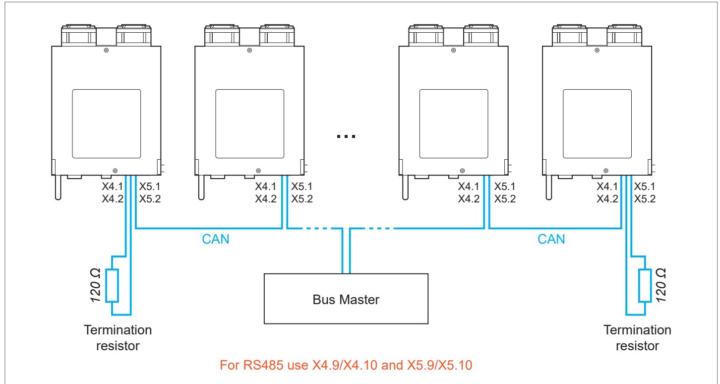
Fig. 25: Use of termination resistors in CAN / RS485 bus
