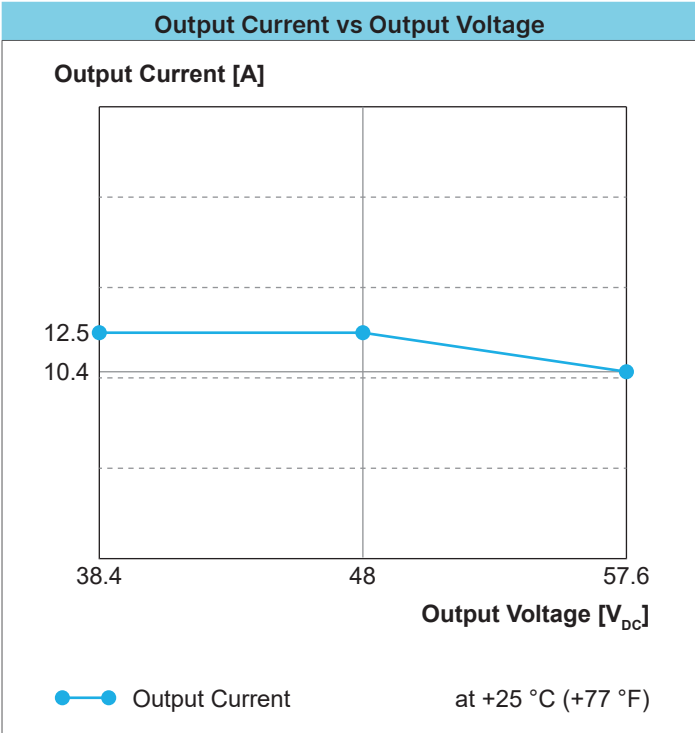
Fig. 22: Output current versus output voltage for W1AC-48DC-300W
