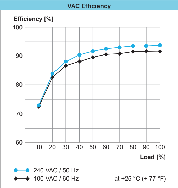
Fig. 23: VAC Efficiency for W1AC-24DC-300W
