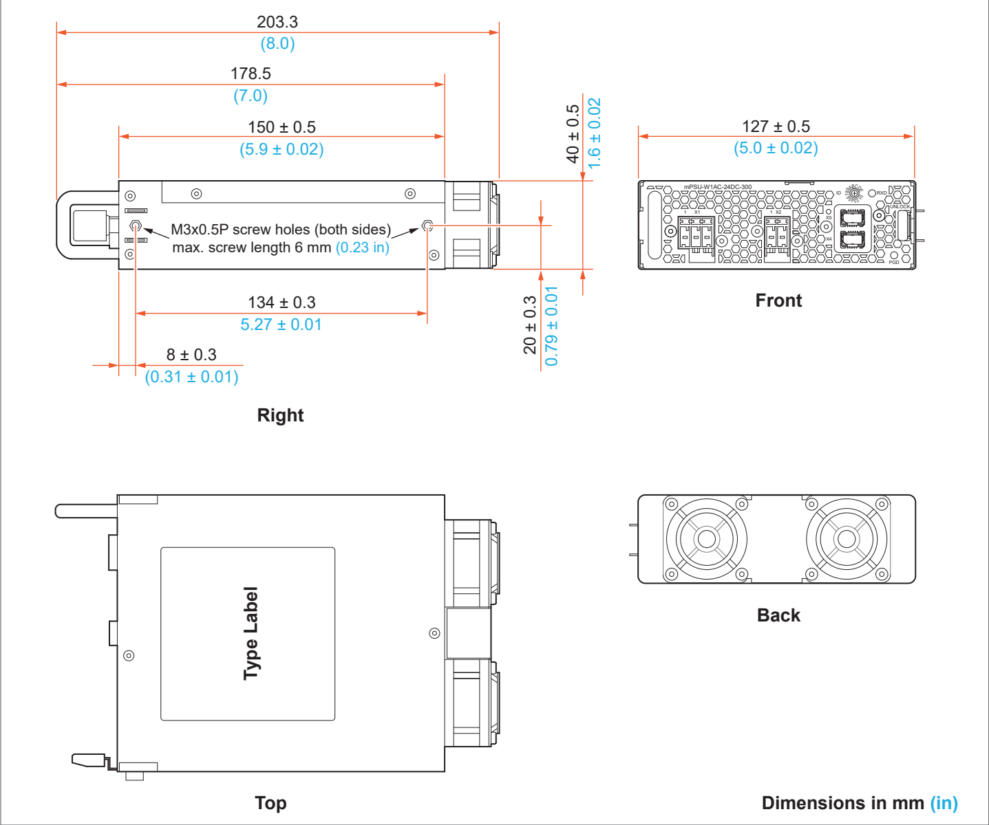
Fig. 17: Dimensions
