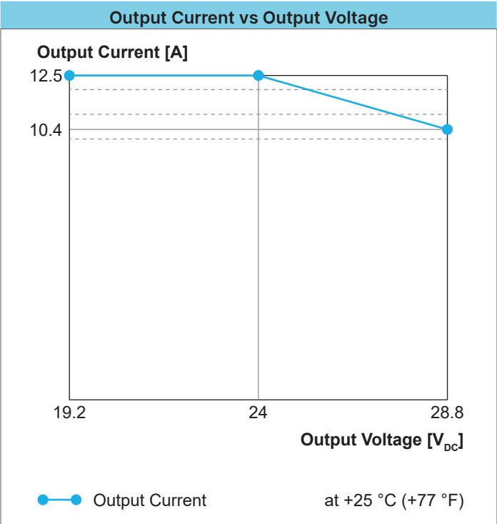
Fig. 21: Output current versus output voltage for W1AC-24DC-300W
