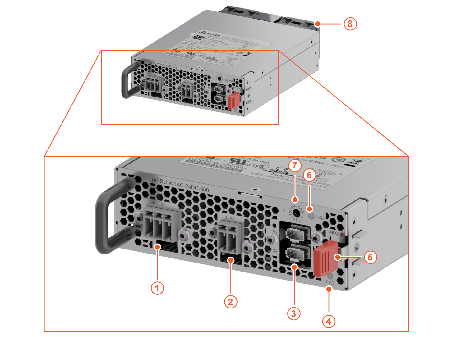
Fig. 1: Components of the mPSU
