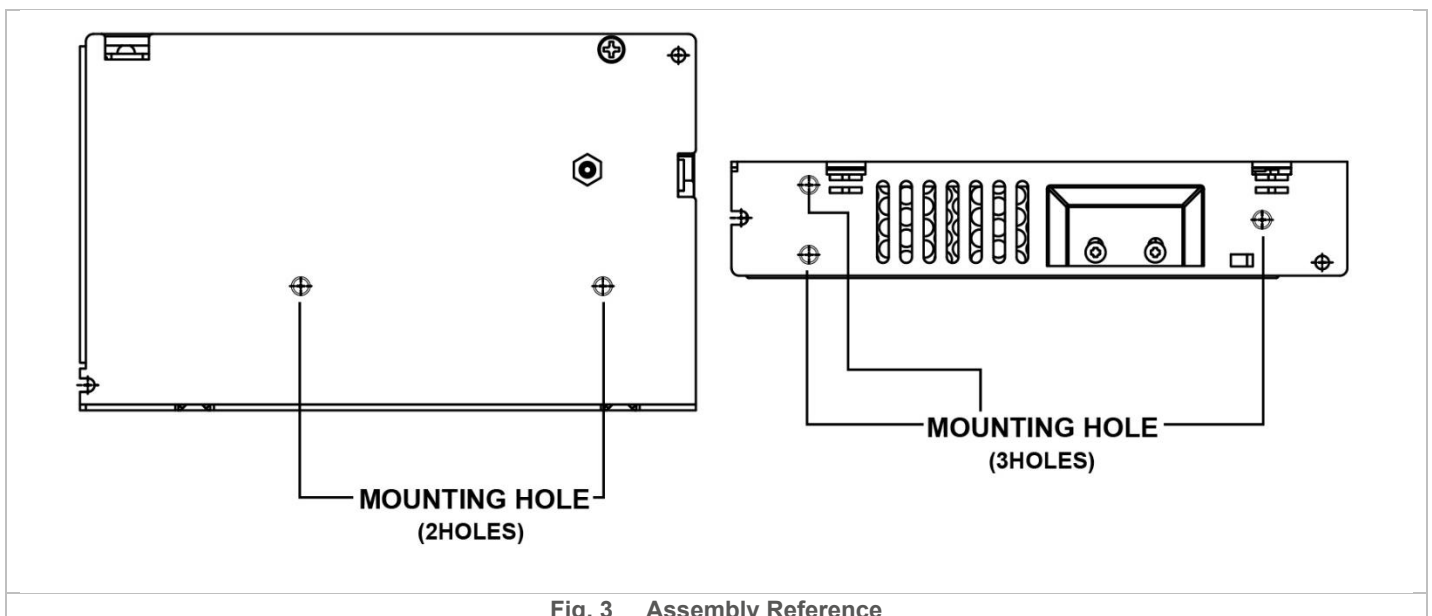
Fig. 3 Assembly Reference
