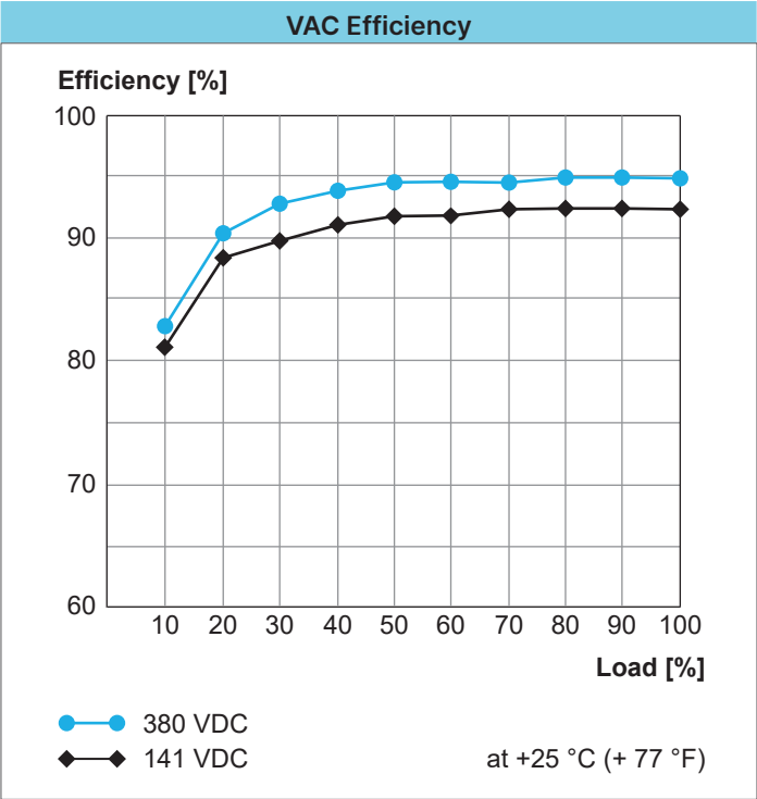
Fig. 23: VAC Efficiency for W1AC-24DC-600W
