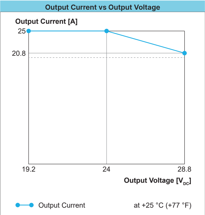
Fig. 21: Output current versus output voltage for W1AC-24DC-600W
