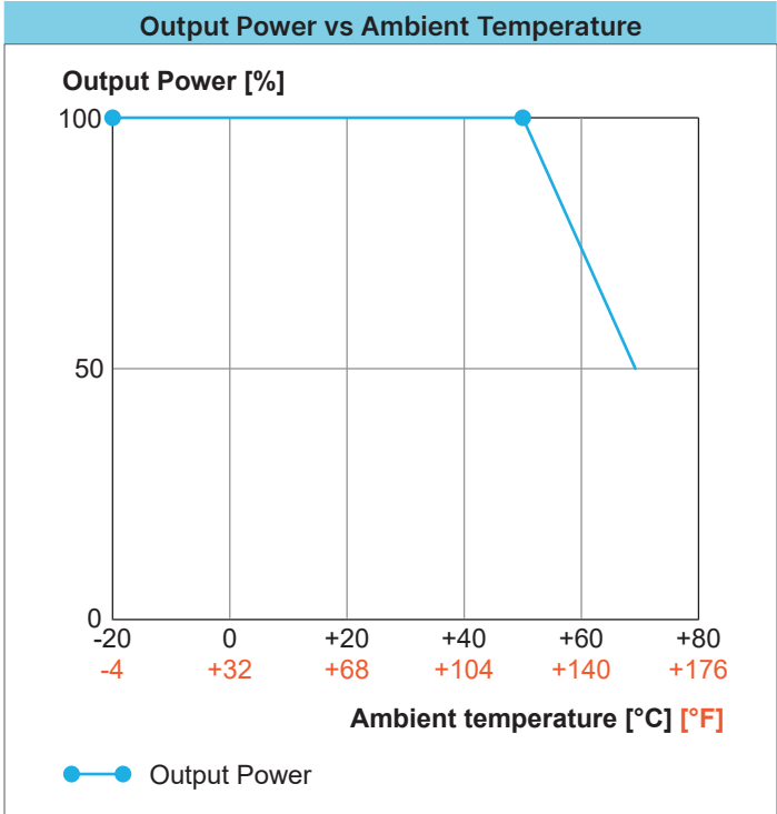
Fig. 20: Output power versus ambient temperature for W1AC-xxDC-600W
