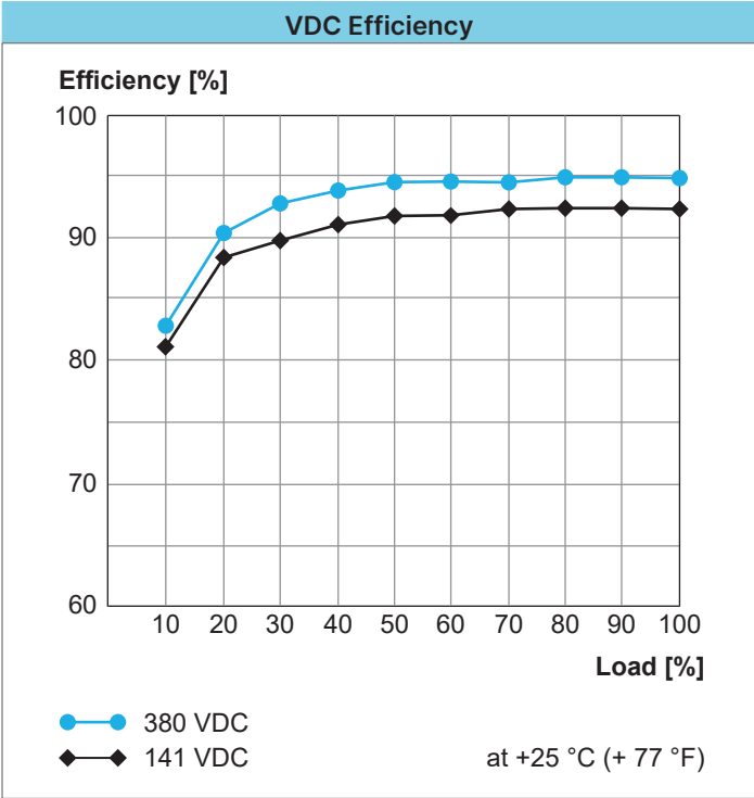
Fig. 24: VDC Efficiency for W1AC-24DC-600W
