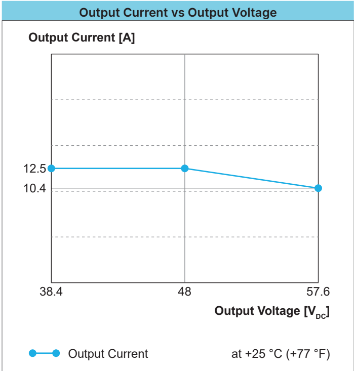
Fig. 22: Output current versus output voltage for W1AC-48DC-600W
