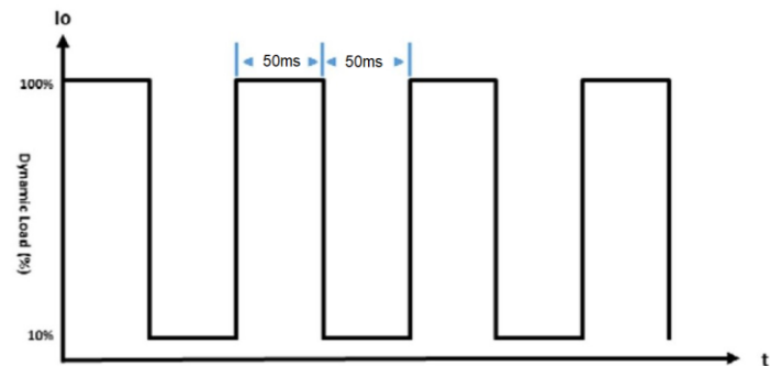
Figure 3. Dynamic Load (10 Hz)
