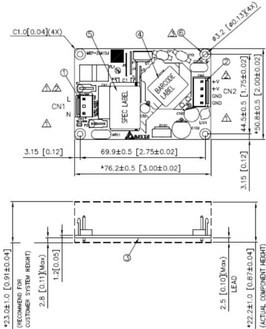
Figure 2. Dimensions
