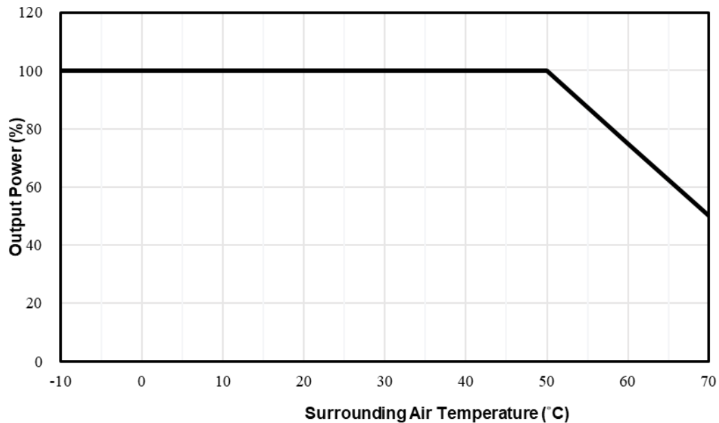
Figure 1. Temperature Power De-rating
